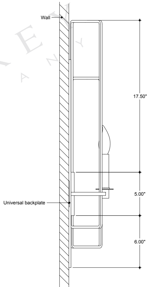
SIDE VIEW
